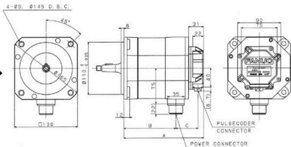
Outline drawing of the motors (standard)
